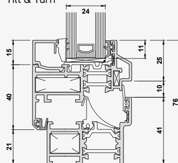
Tilt & Turn
