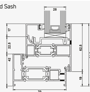
Tilt & Turn
