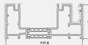
Double Track
