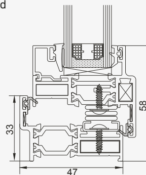
Tilt & Turn
