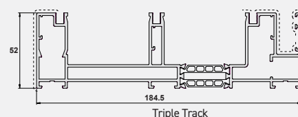
Triple Track
